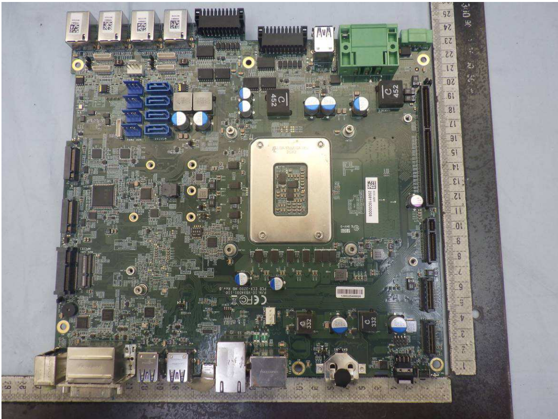
Top side view - 2 of main board
